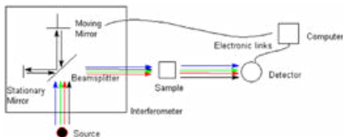
Figure 1: FTIR principle
