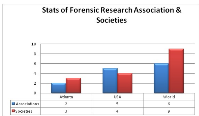
Figure 1: Statistical Analysis
